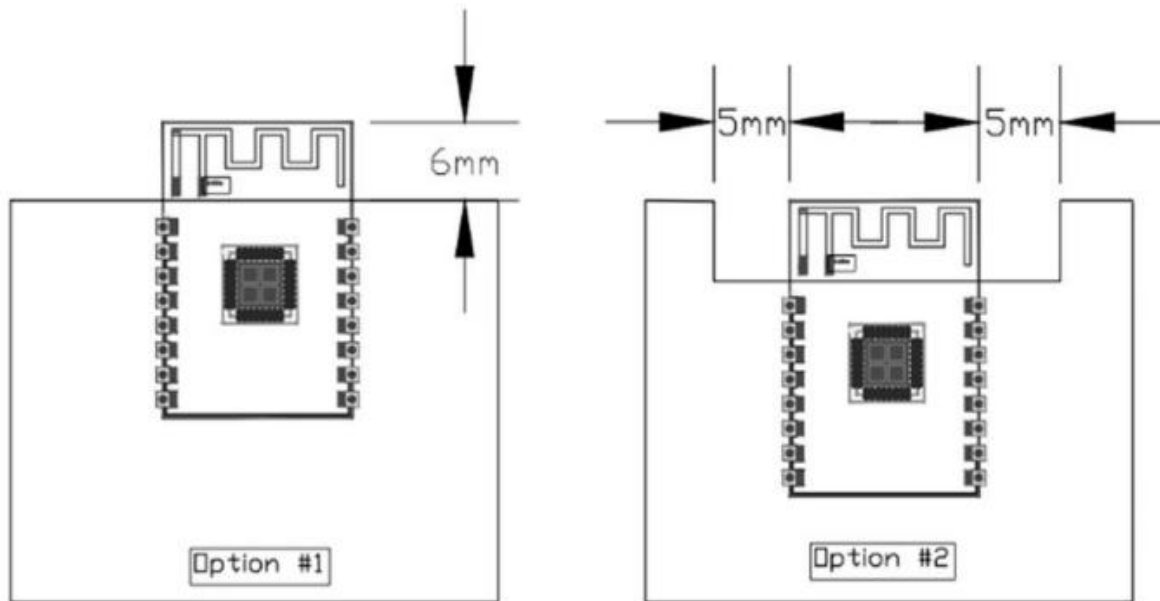
Figure 11 Schematic diagram of antenna layout
