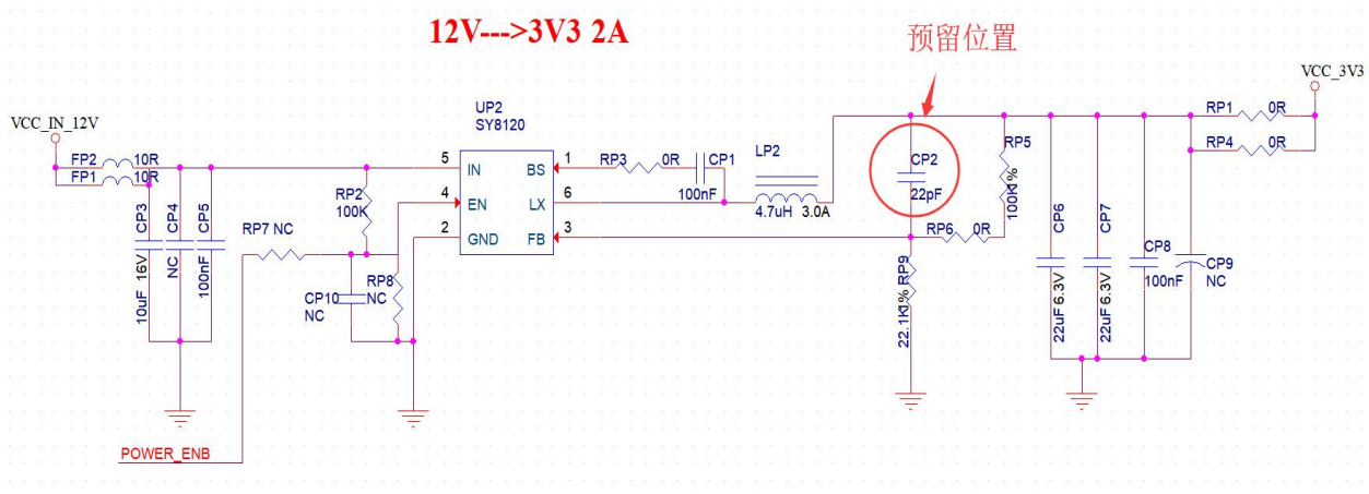
Figure 12 DC-DC step-down circuit diagram
