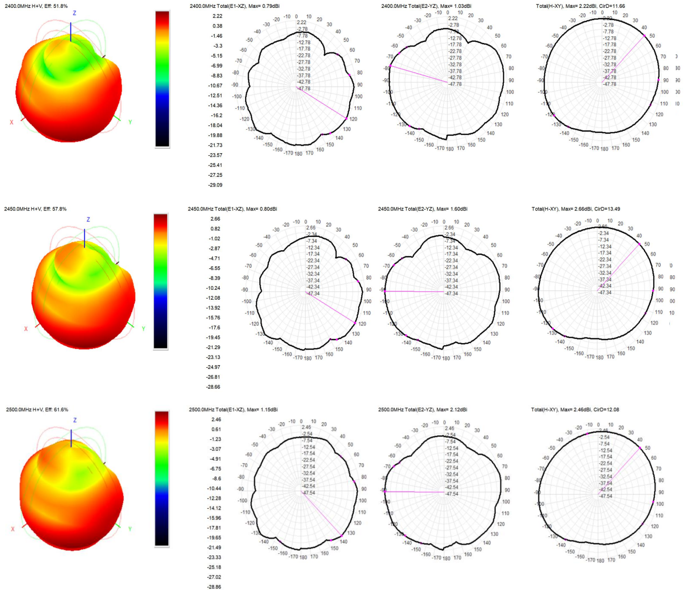
Figure 9 Antenna field pattern
